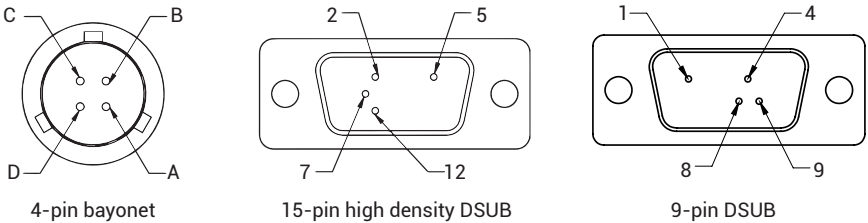
Diagram 2: Transducer pin out
