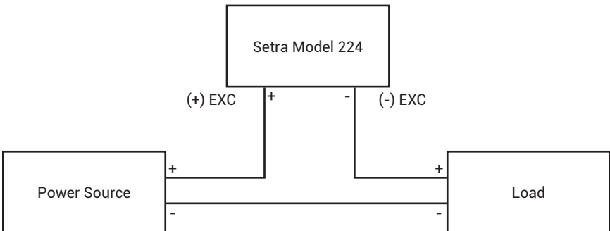
Diagram 4: Current wiring diagram
