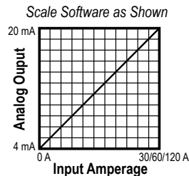
Figure 7: CTCG420NN Linear Output
