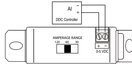
Figure 8: CTCGV05NN Wiring
