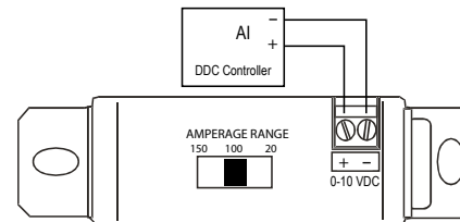
Figure 10: CTCGV10NN Wiring
