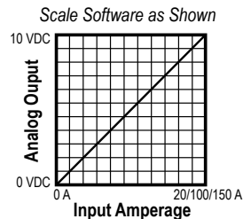
Figure 11: CTCGV10NN Linear Output
