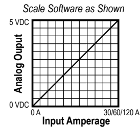
Figure 9: CTCGV05NN Linear Output
