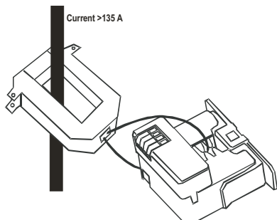
Figure 4: CSC with CT Transformer
