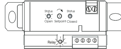
Figure 8: Status Open, LED On
