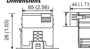
Figure 1: CSC Dimensions mm (in.)
