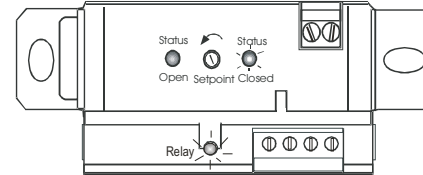
Figure 7: Status Closed, LED On
